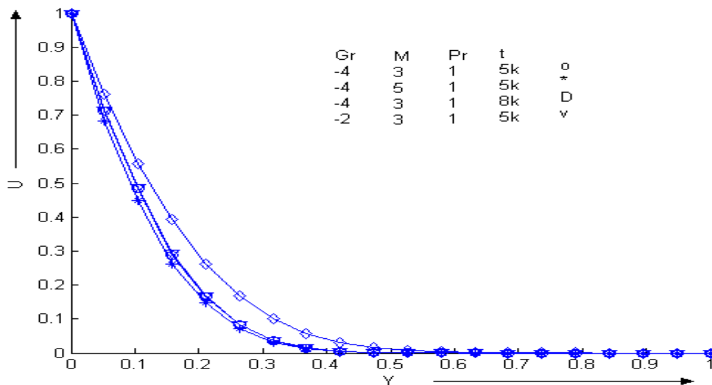
Fig (6) Velocity profiles for Pr < 1 and different Gr , t , m (for heating of plate)
