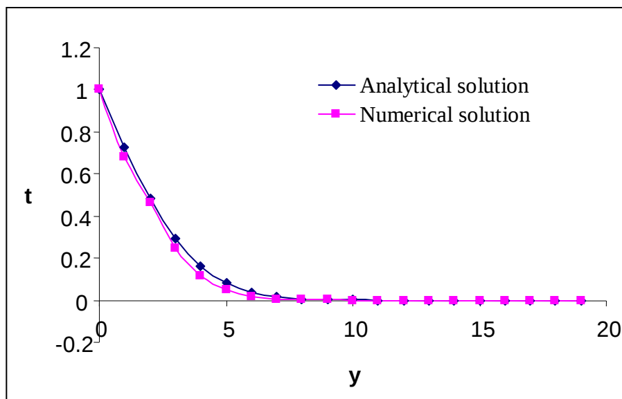
Fig.3. Comparison of Velocity when P_r=6.75
